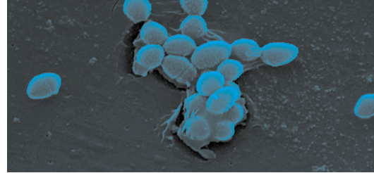
Enterococcus faecalis
